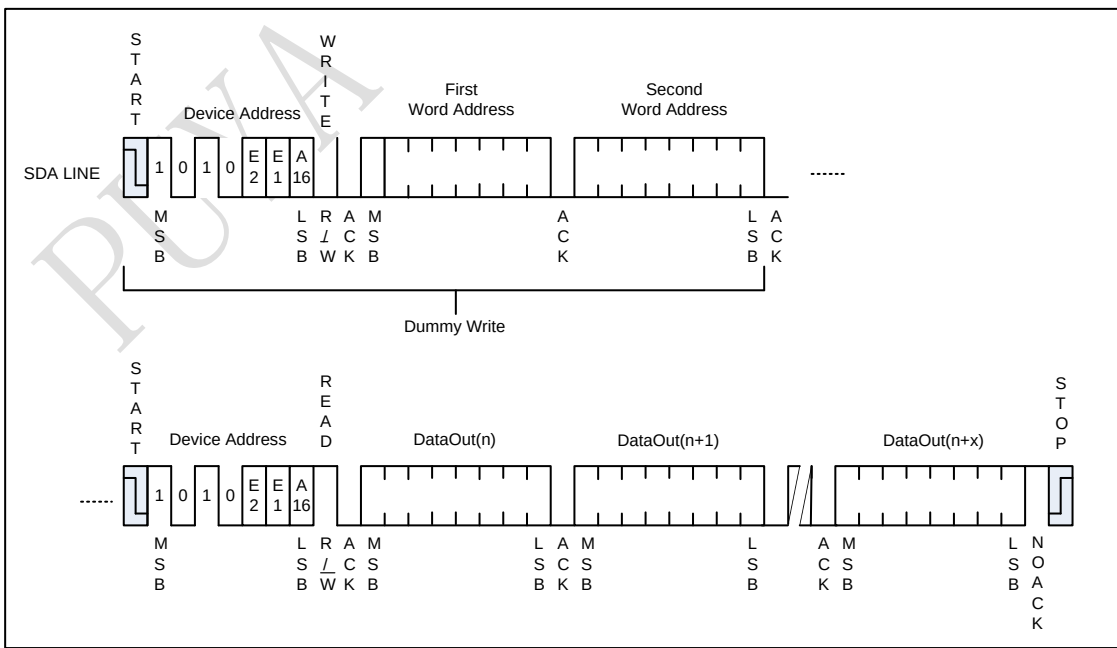
Figure 5-5 Sequential Read
