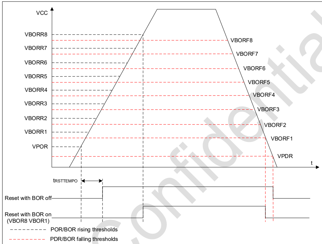
Figure 2-3 POR/PDR/BOR threshold
