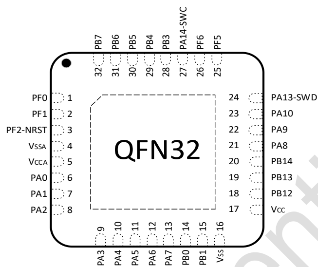
图 3-1 QFN32 PY32M070K1xU7 Pinout1 (Top view)
