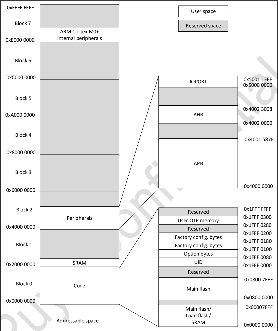
Figure 4-1 Memory map
