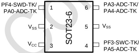
Figure 3-9 SOT23-6 Pinout1 PY32T02061xV7 (Top view)
