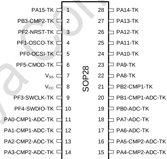
Figure 3-4 SOP28 Pinout2 PY32T020G2xS7 (Top view)
