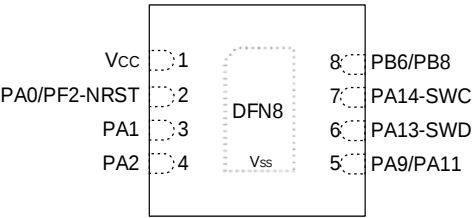
图 3-9 DFN8(2*2) Pinout1 PY32F031L1xD6 (Top view)
